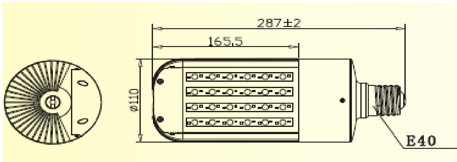
LAMP DIMENSION
